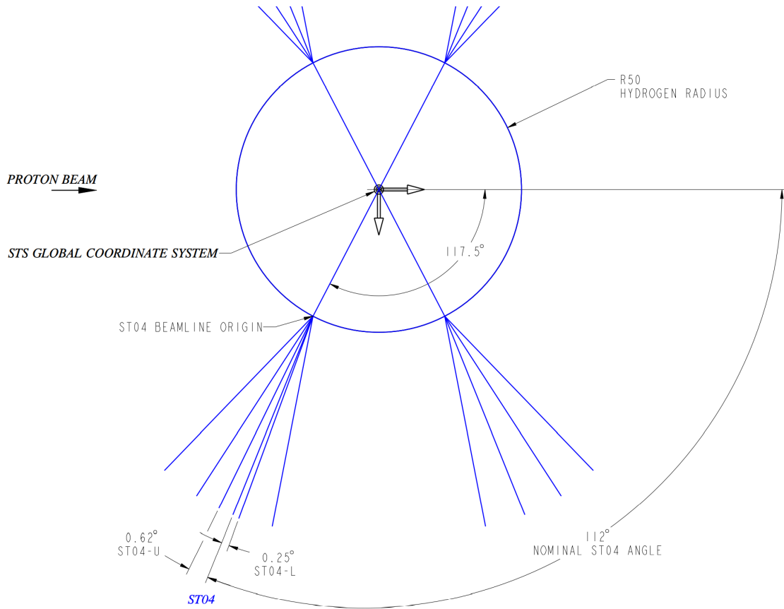
Figure 18. ST04-U and ST04-L Plan View (dimensions in mm, angles are not to scale for clarity).
