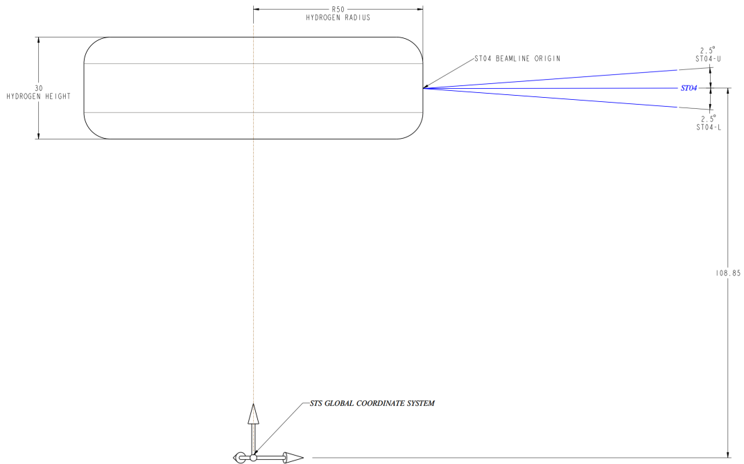
Figure 19. ST04-U and ST04-L Vertical Cross-section through ST04 Layout (dimensions in mm, angles are not to scale for clarity).
