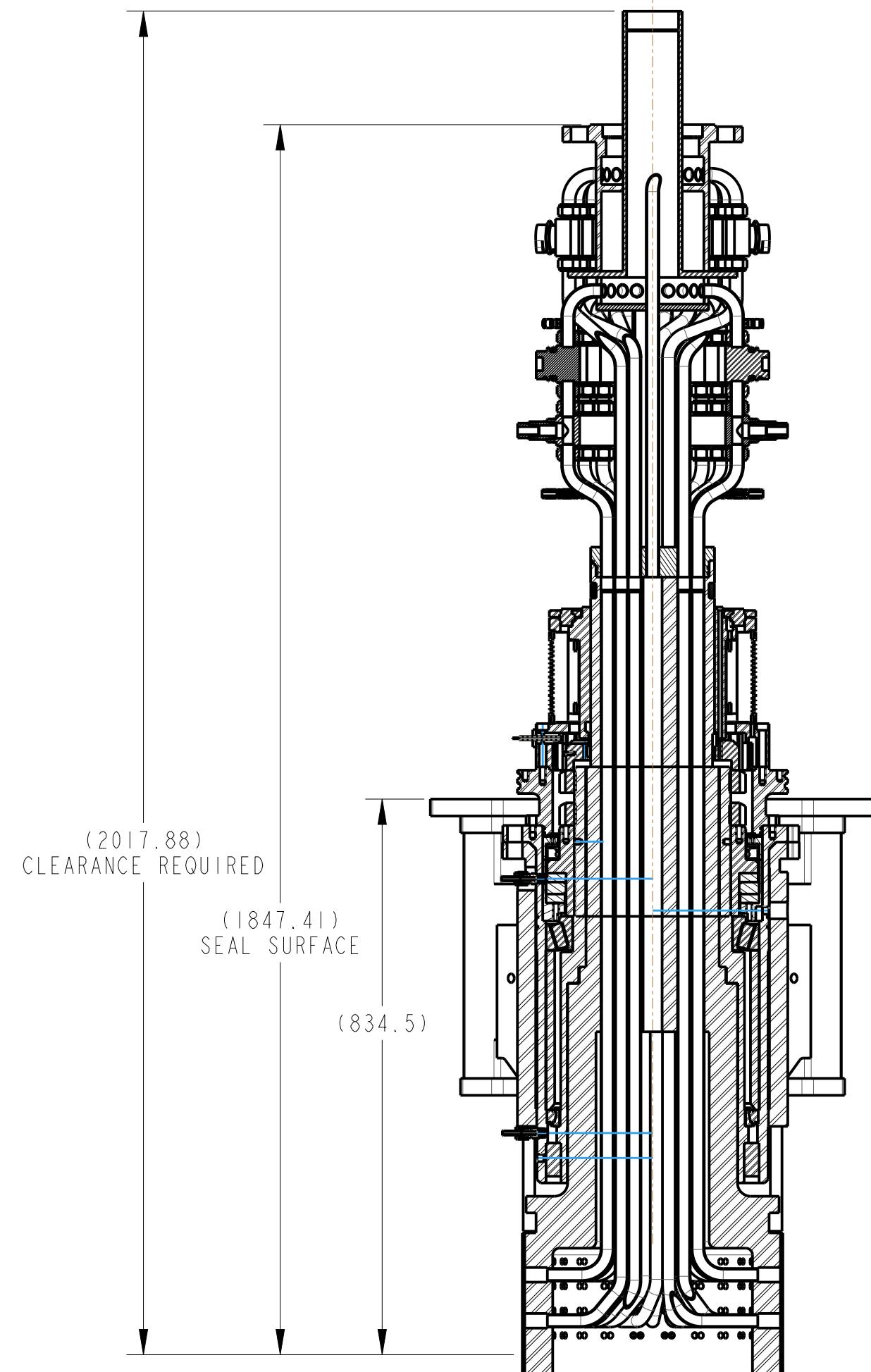
WATER ROTARY UNION REMOVED SECTION B-B SCALE 1:8
