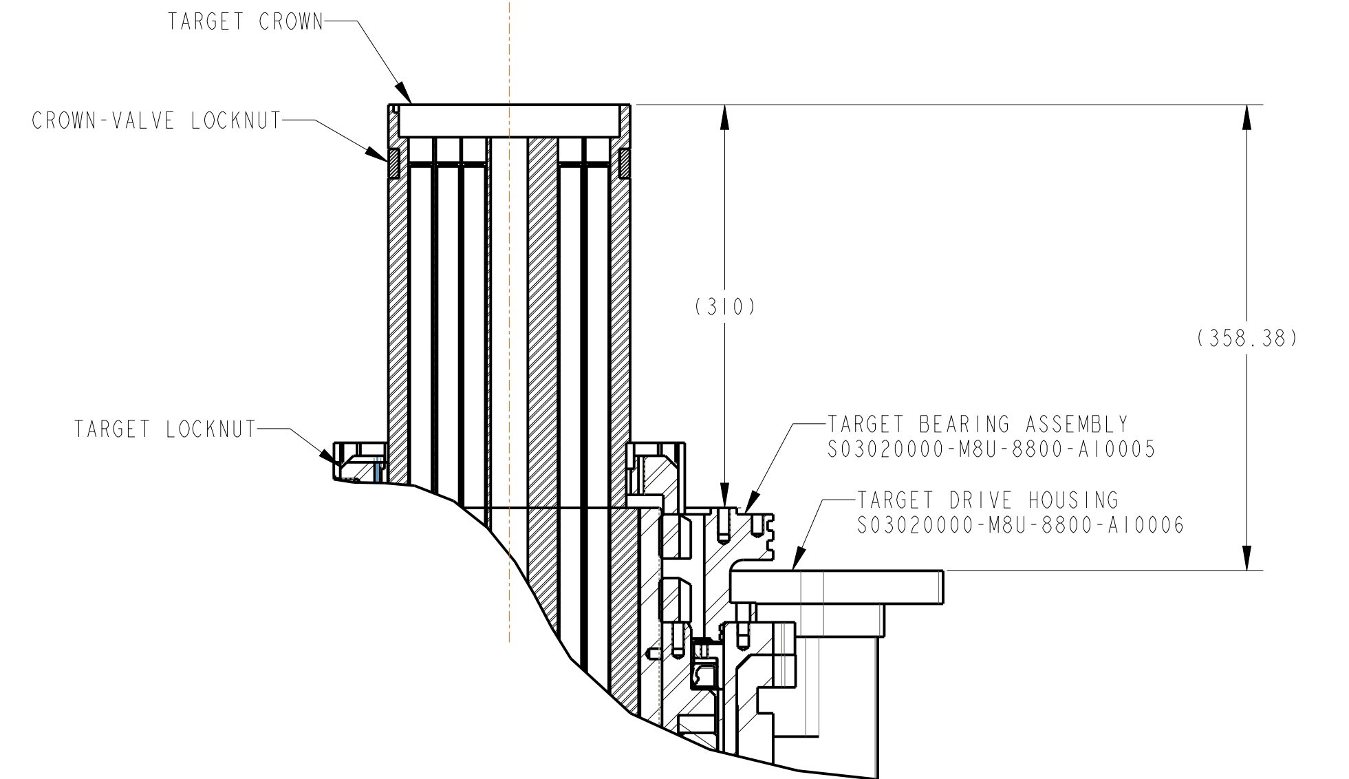
DETAIL N SCALE 1:4
