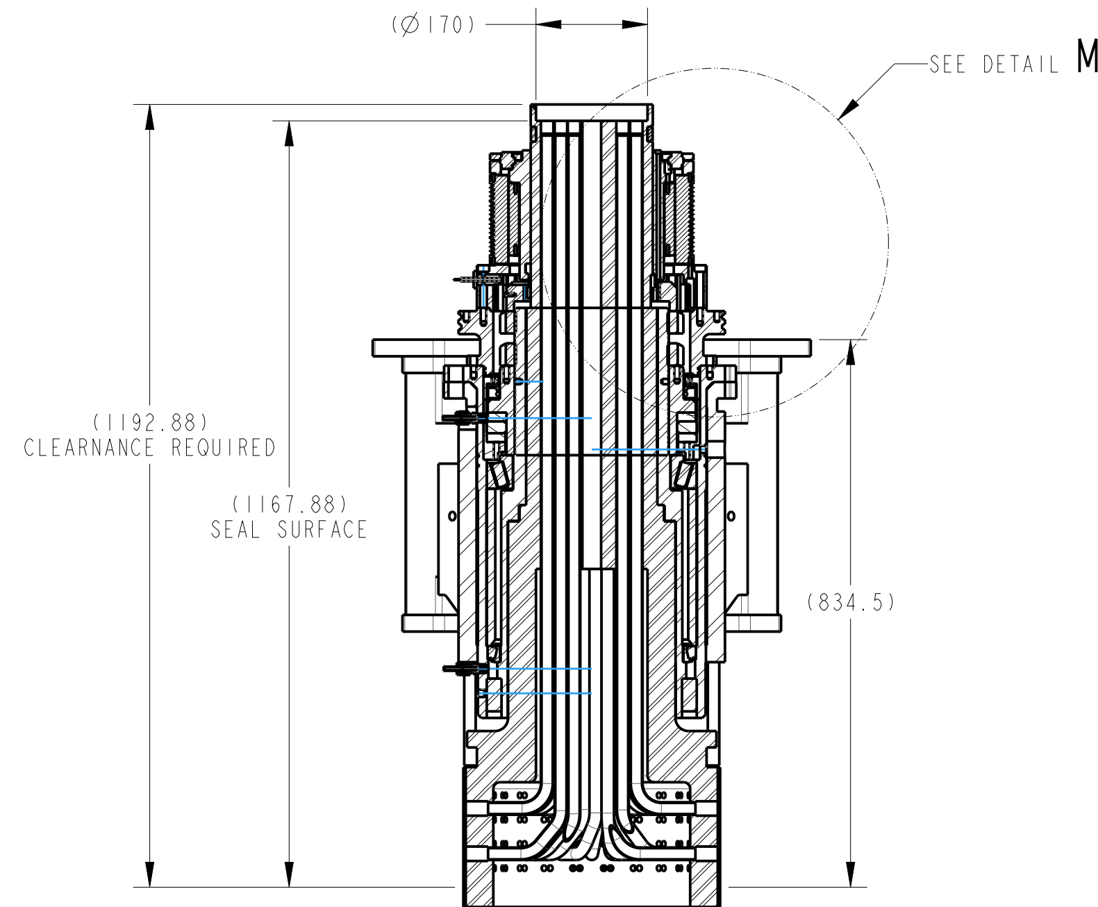
VALVE CROWN ASSEMBLY REMOVED SECTION B-B SCALE 1:8
