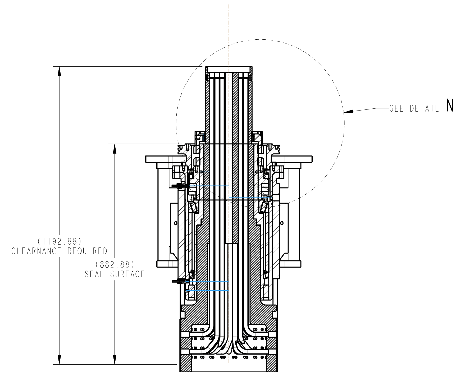
TARGET MOTOR AND MOUNT REMOVED SECTION B-B SCALE 1:8
