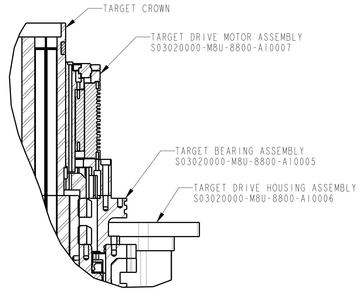
DETAIL M SCALE 1:4
