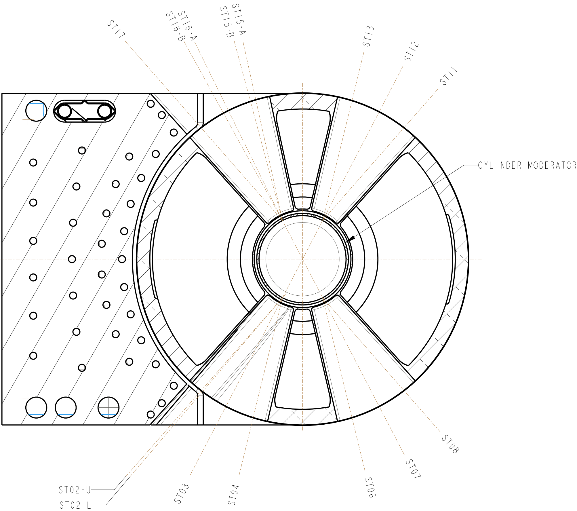
SECTION AT CYLINDER MODERATOR BEAMLINE REFERENCE
