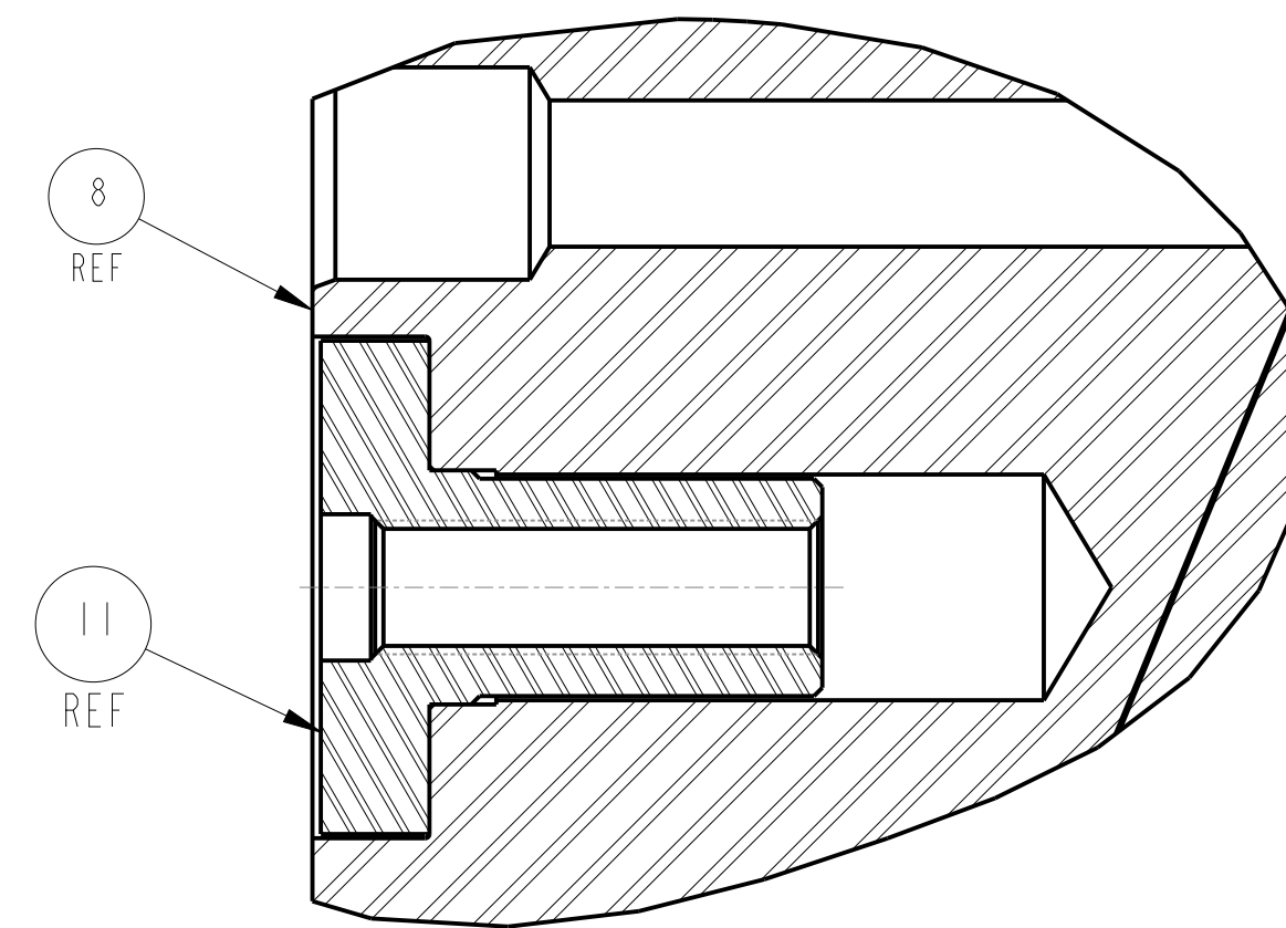
SECTION G-G (SH1) SCALE 1:1
