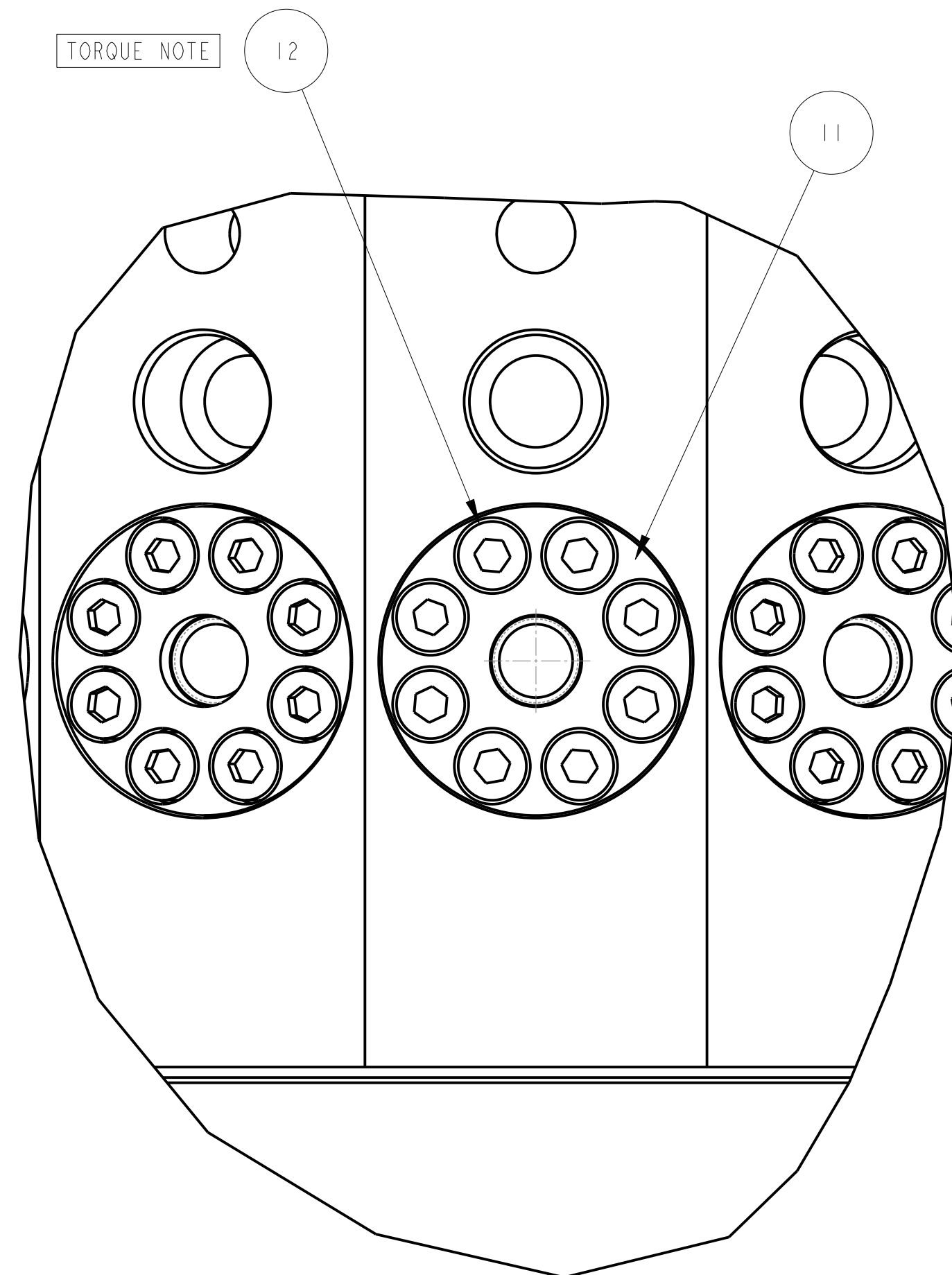
DETAIL H SEGMENT BOLT ADAPTOR (SH1) SCALE 1:1
